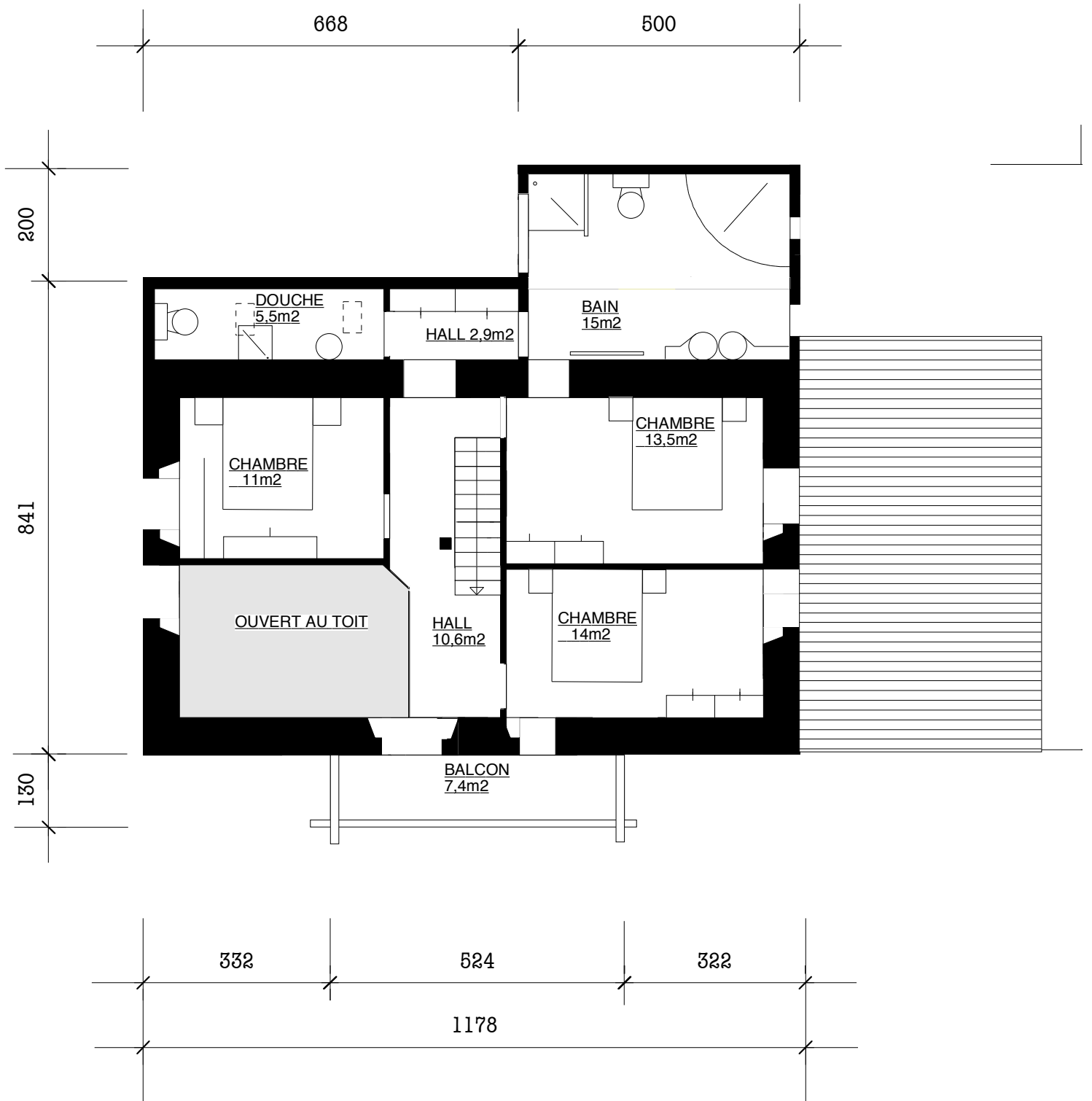
PLAN COMBLES 1/100
